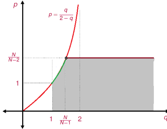
FIGURE 1. Regions of nonexistence of positive supersolutions which do not blow up at infinity in the plane q, p .
